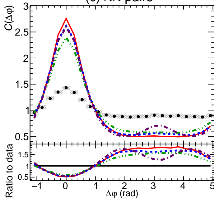
(c) \Lambda\bar{\Lambda} pairs
