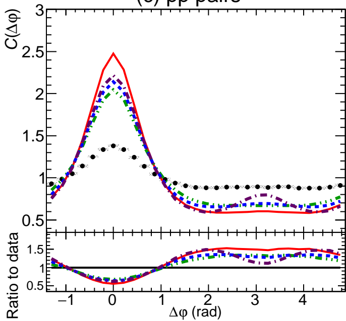
(c) p\bar{p} pairs
