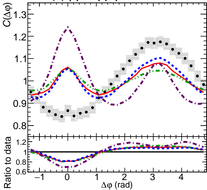
(c) pp + \bar{p}\bar{p} pairs
