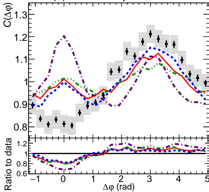
(c) \Lambda\Lambda + \bar{\Lambda}\bar{\Lambda} pairs
