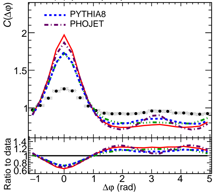
(b) p\Lambda + \bar{p}\Lambda pairs
